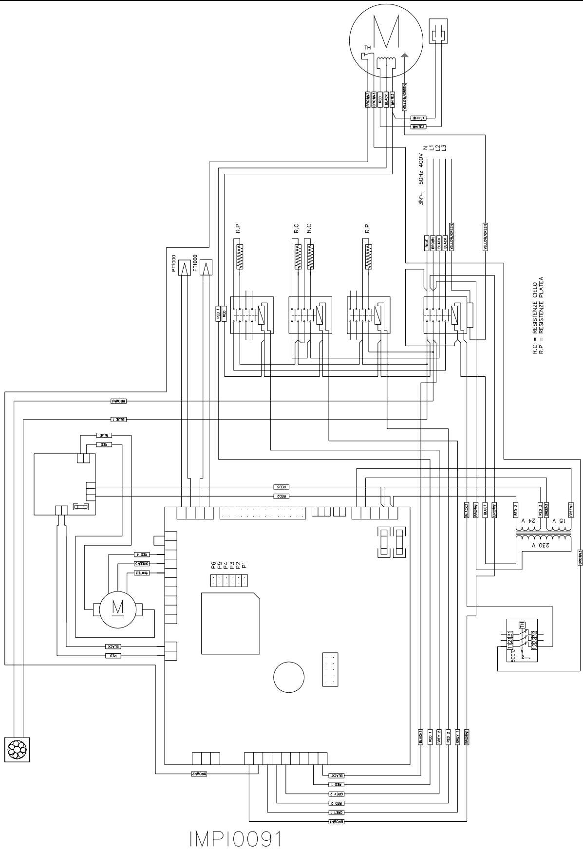
Fig. 10-4 Wiring diagram DPZ6030E - 400 Vac. ~ 3+N 50-60Hz
